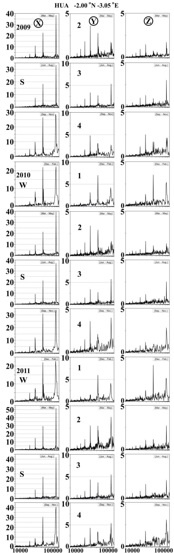
Figure 2. Average seasonal spectra in HUA
